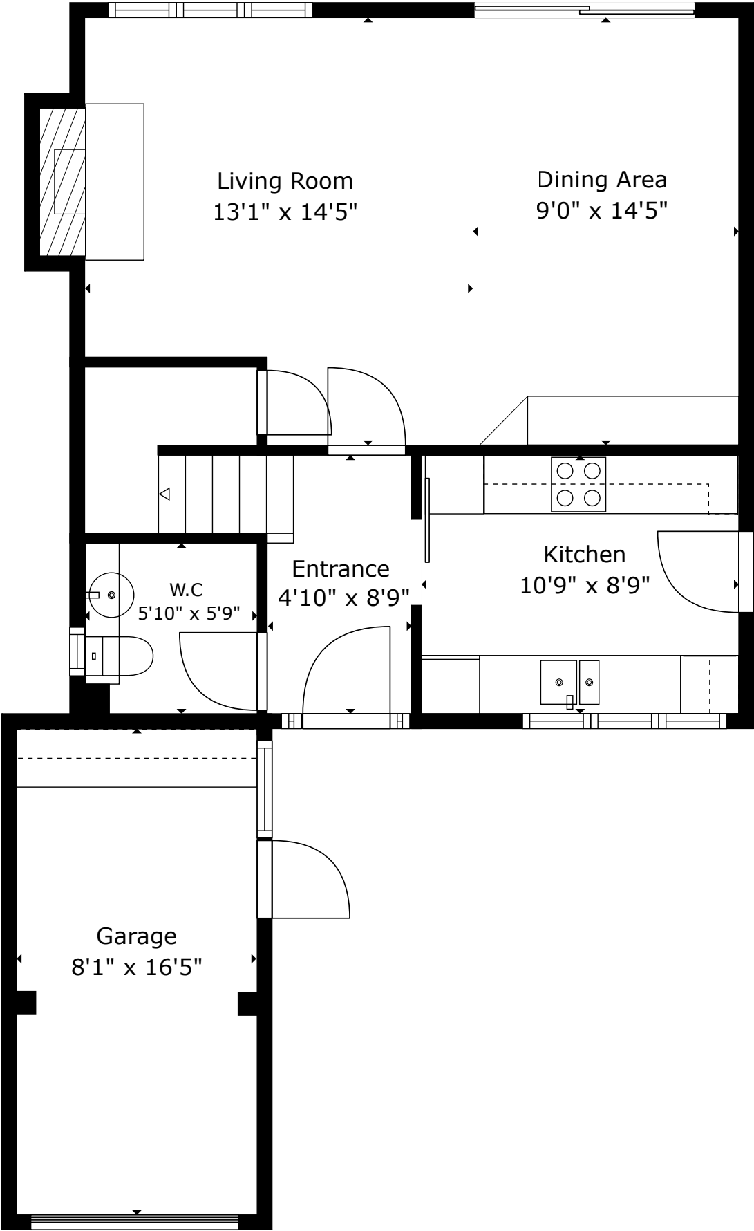
► Ground Floor
