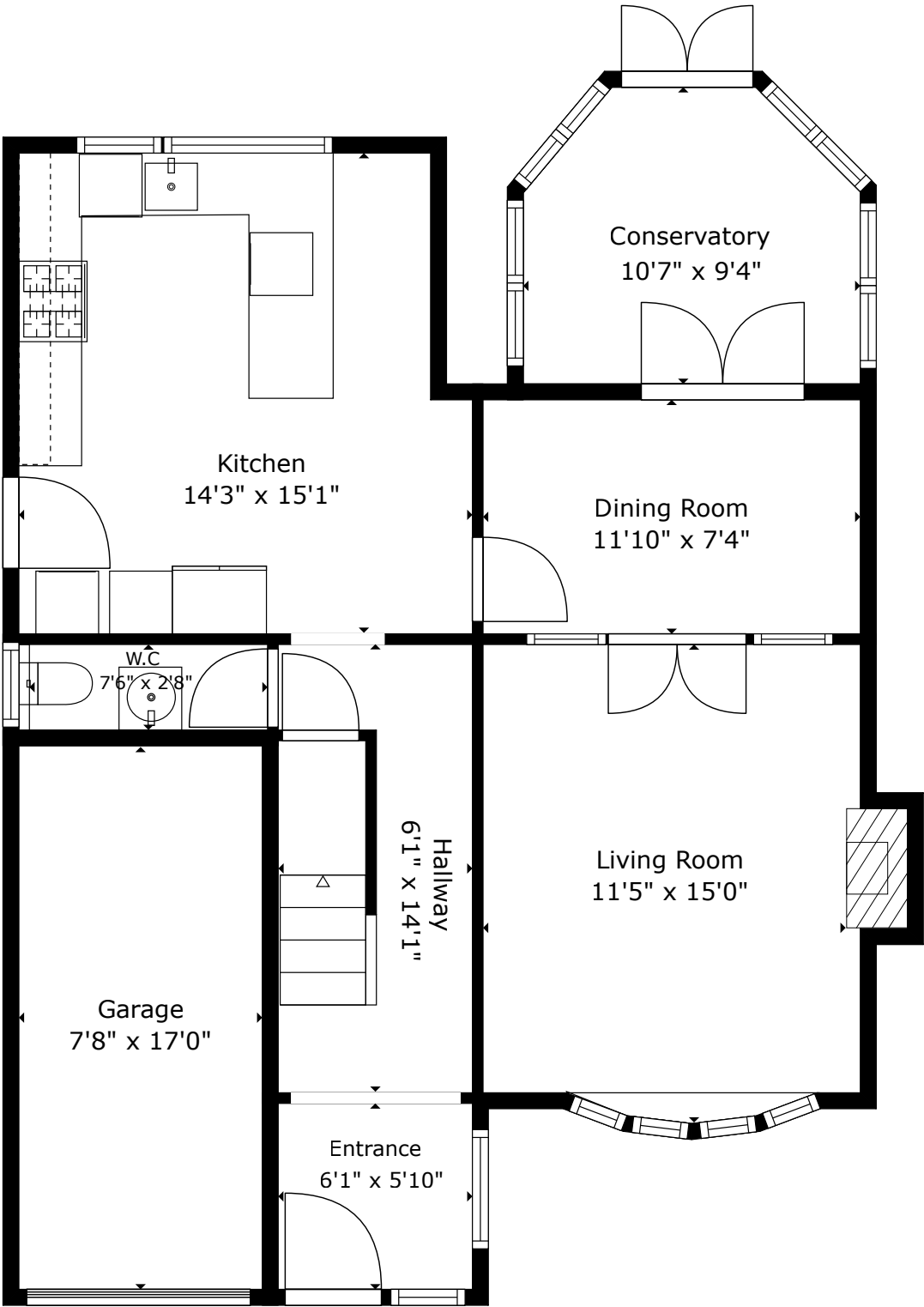
► Ground Floor
